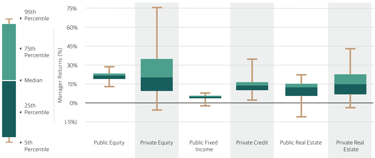
Dispersion of Fund Performance, Manager Returns Over a 5 Year Period
